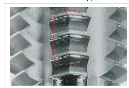
Wear after 360 holes tapped
